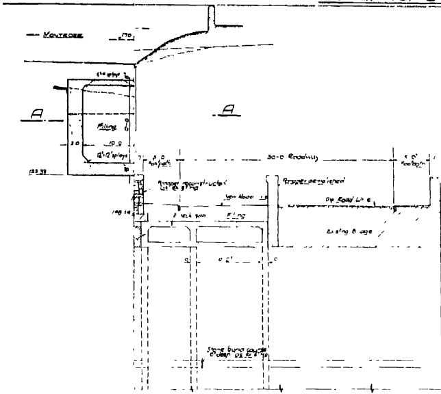
CROSS SECTION AT CROWN
